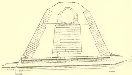
Cochituate Aqueduct.
